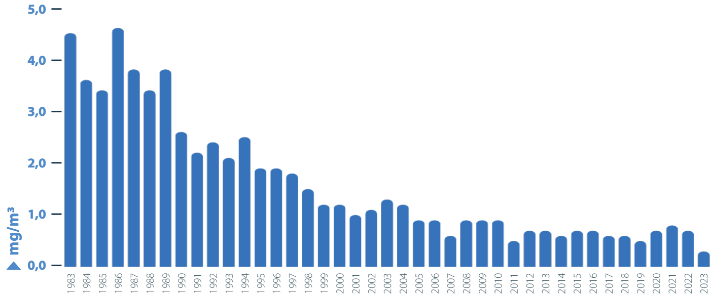
Figura 5.6: CO – media annua
