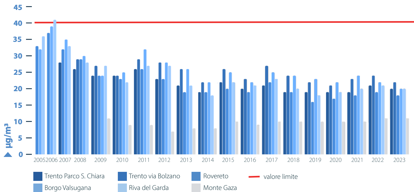
Figura 5.4: PM10 – media annua
