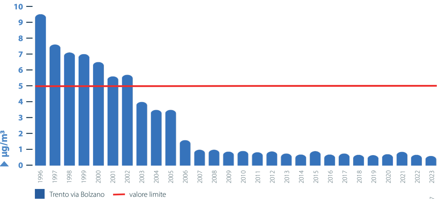
Figura 5.8: C 6 H 6 – media annua
