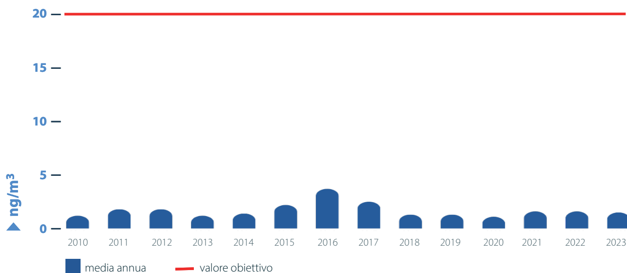
Figura 5.12: Ni – media annua
