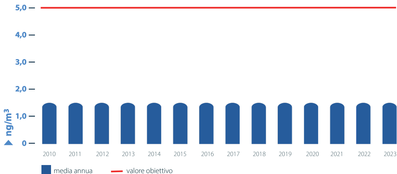
Figura 5.11: Cd – media annua
