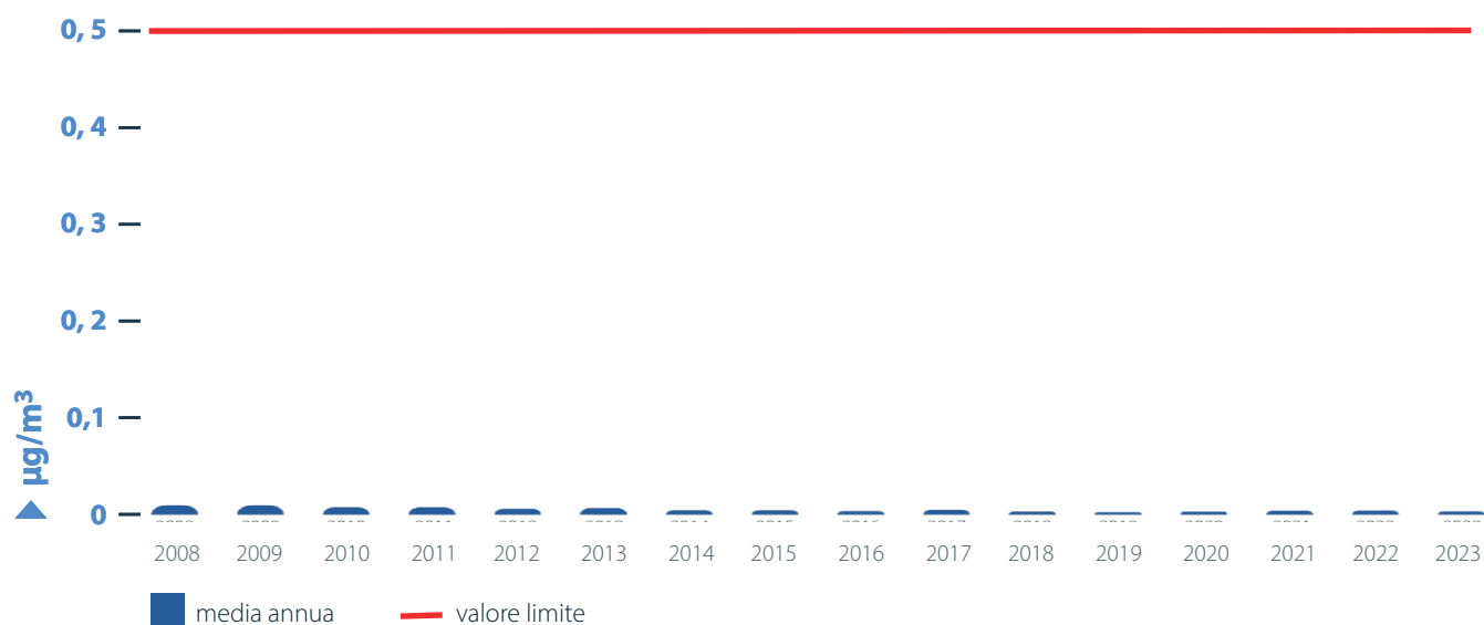
Figura 5.9: Pb – media annua
