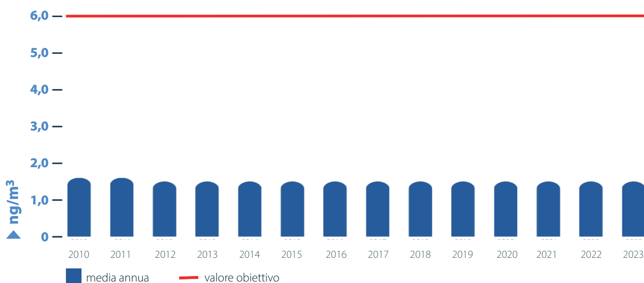
Figura 5.10: As – media annua
