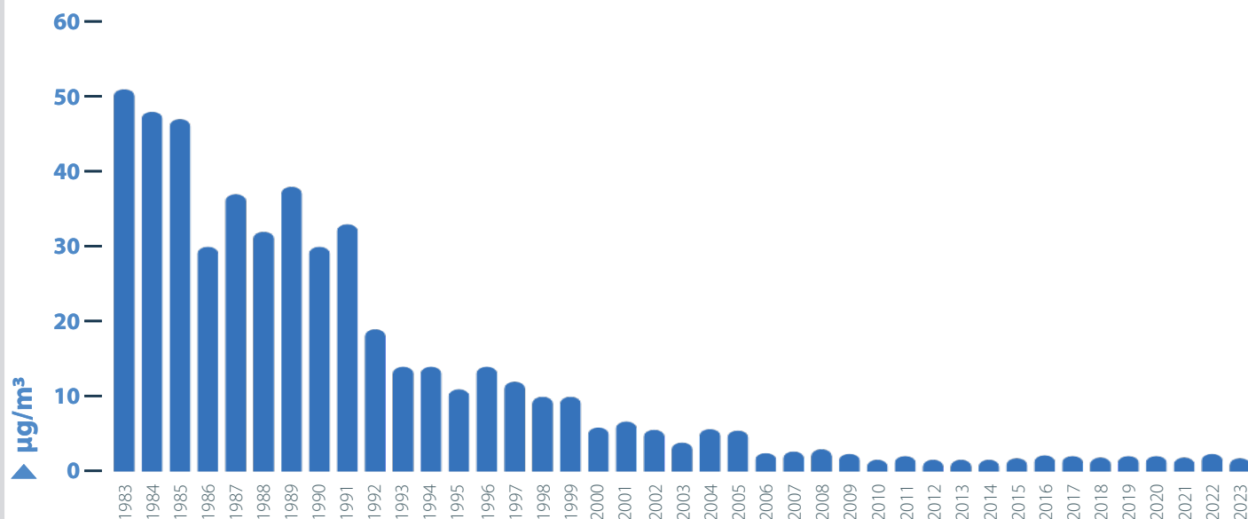
Figura 5.7: SO 2 – media annua
